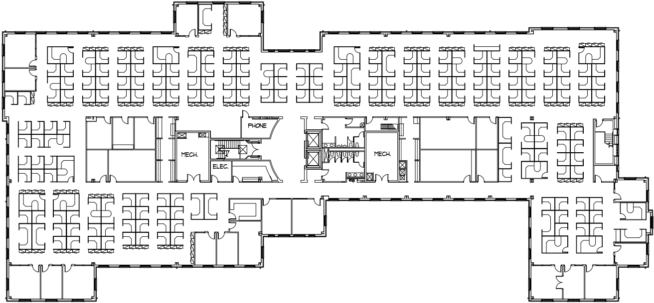
Third Floor, Existing Conditions Plan
