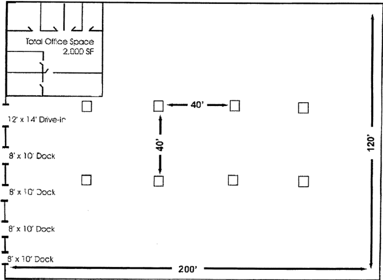
Floor Plan
